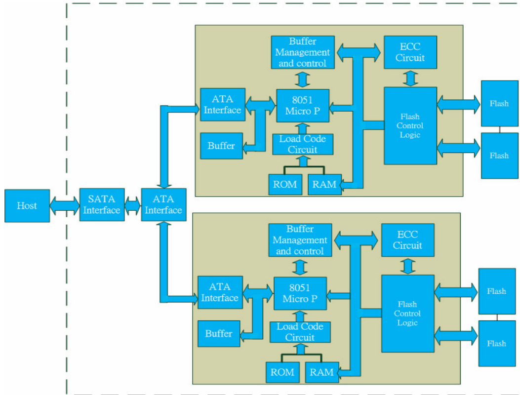
Figure 2: InnoDisk FiD 2.5" SATA 6000 Block Diagram
